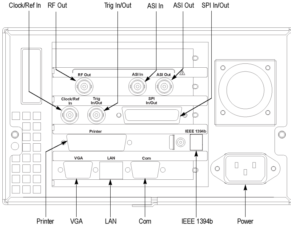
Figure 2: RTX100B rear panel
