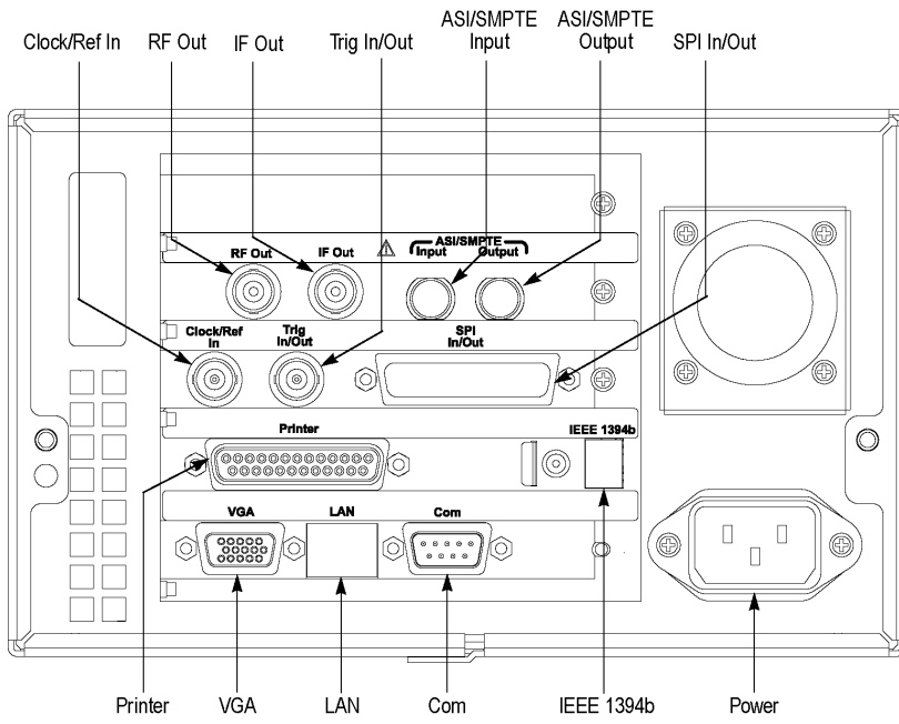
Figure 1: RTX130B rear panel
